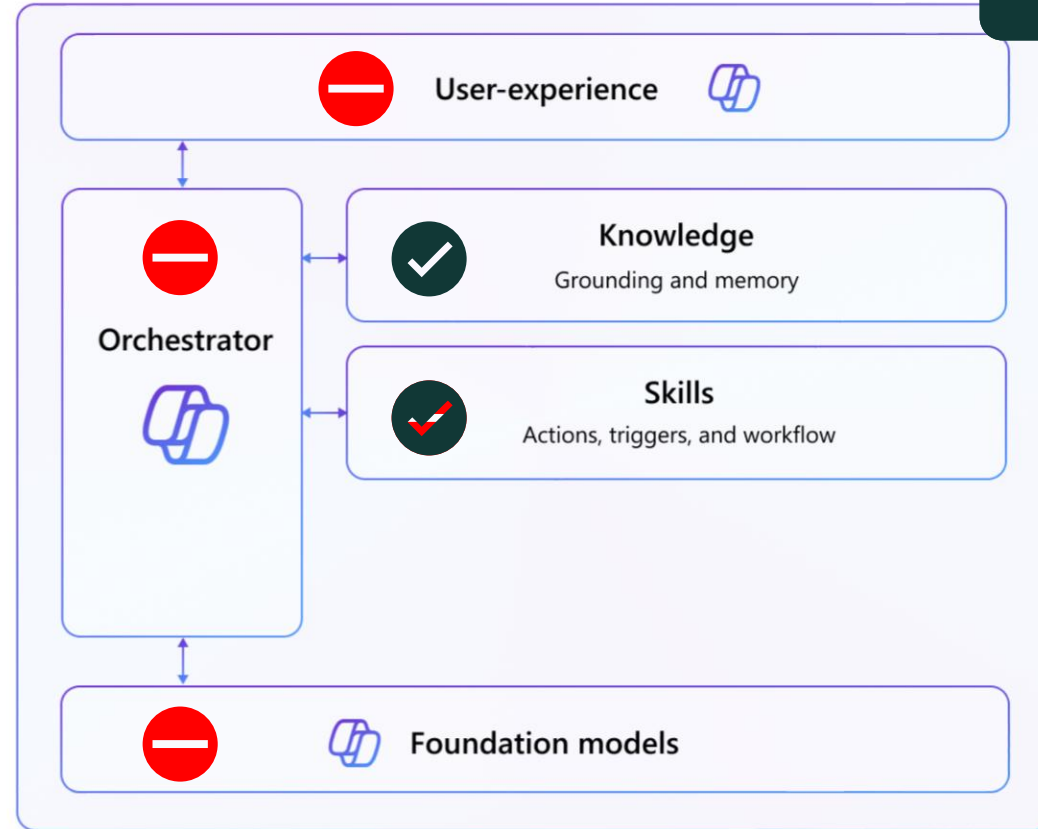
Anatomy of Declarative agent
